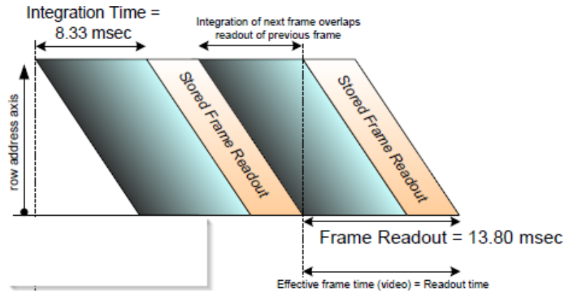
Figure 2.5a: Rolling Shutter Mode with 8.33 ms exposure time.
