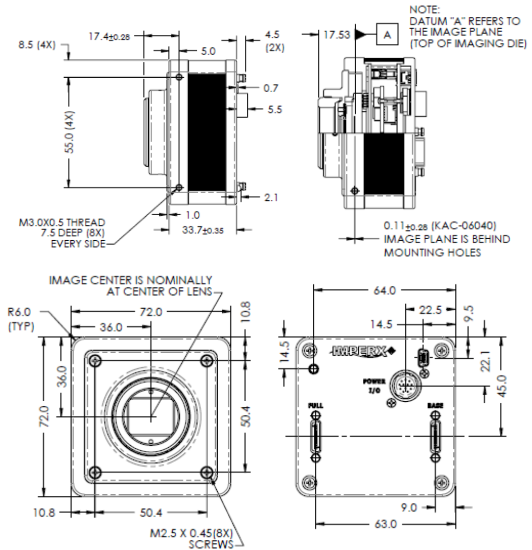
Figure 1.7b: C2880 Mechanical Drawings (C-Mount)
