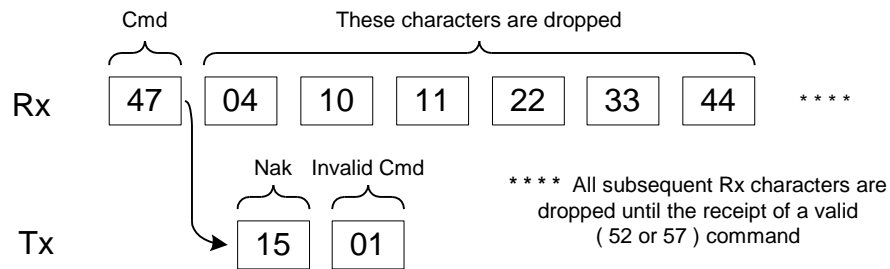
Figure 3.3a: Invalid command error
