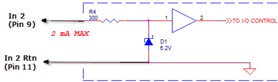
Figure 2.15b: IN 2 electrical connection
