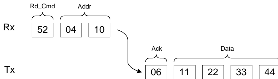
Figure 3.4: Normal read cycle
