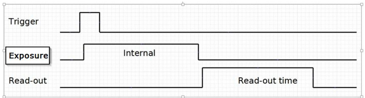
Figure 2.6a: Standard Trigger Mode (Internal Exposure Control)
