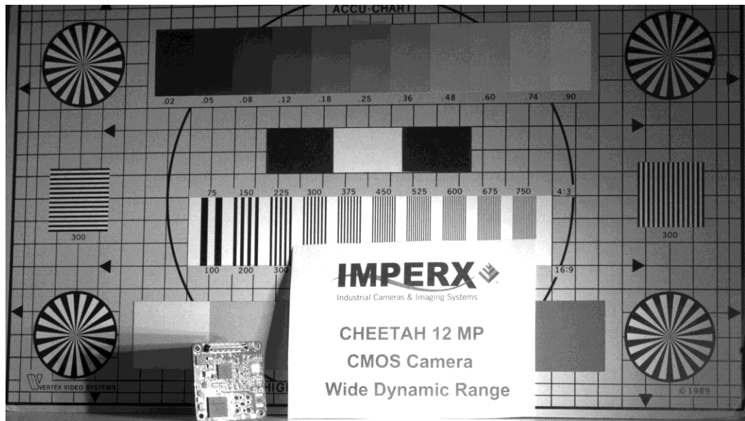
Figure 2.8b: WDR mode enabled
