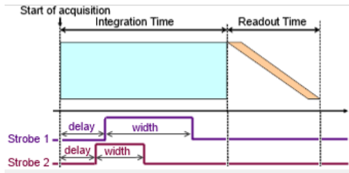
Figure 2.7: Strobe positioning with respect to exposure start
