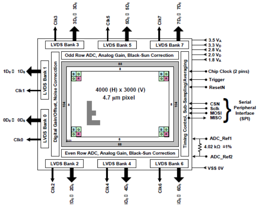
Figure 1.1: CMOS image sensor architecture
