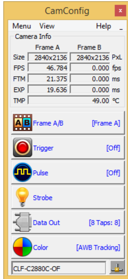
Figure 4.2: CamConfig GUI
