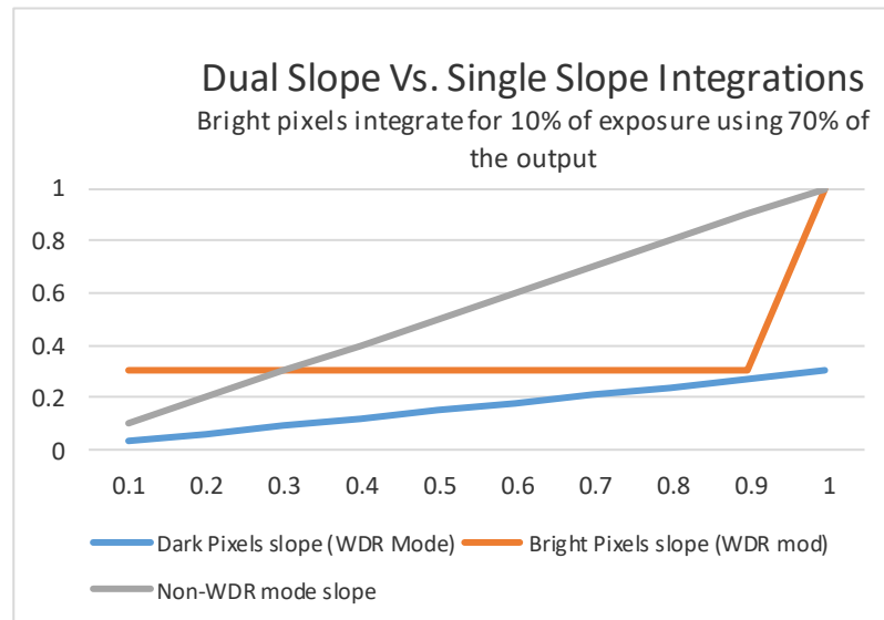
Figure 2.9: Dual Slope vs Single Slope Integration
