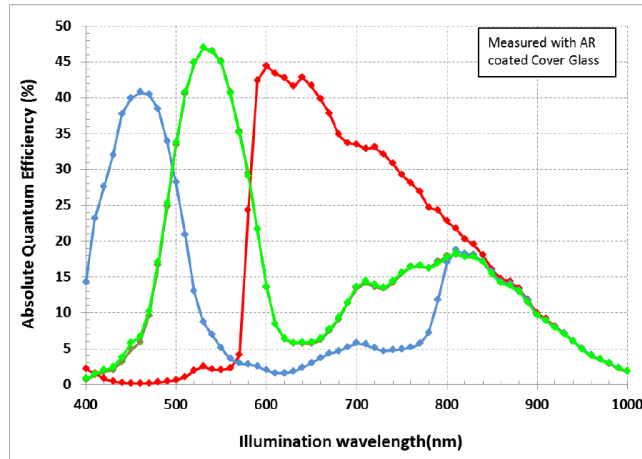
Figure 1.2b: KAC-XX040 CMOS typical color spectral response. (Color with microlens and cover glass)
