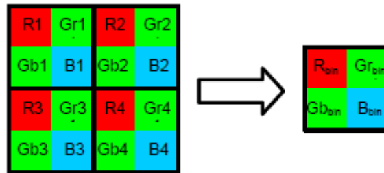
Figure 2.3: Principle of 4:1 averaging for Bayer Color Filter Pattern
