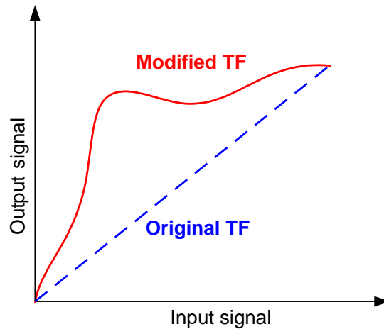
Figure 2.18: Custom LUT
