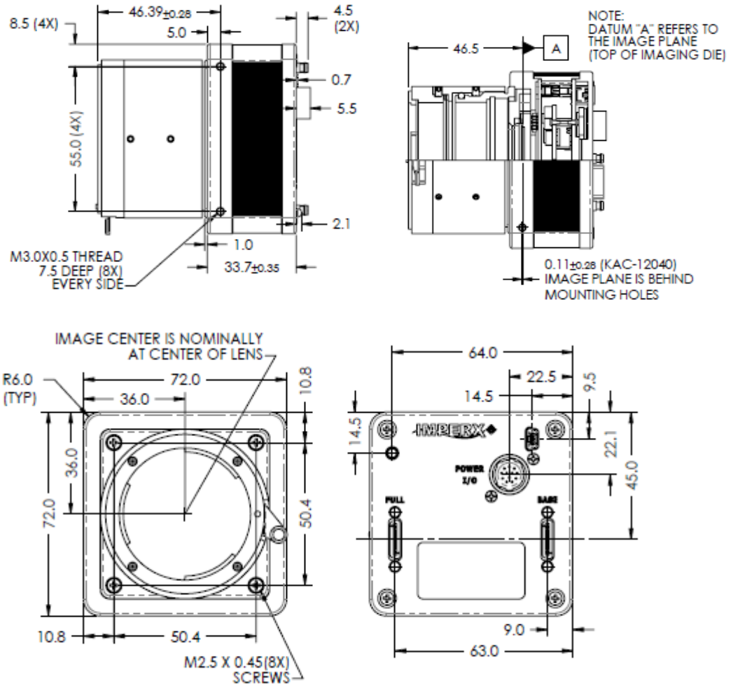
Figures 1.7a: C4080 Mechanical Drawings (F-Mount)
