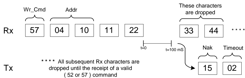
Figure 3.3b: Rx timeout error
