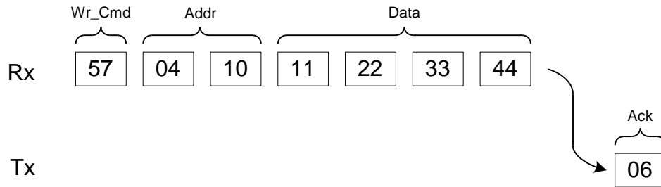
Figure 3.2: Normal write cycle
