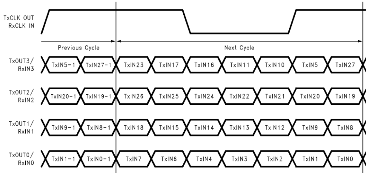
Figure 1.5: Camera Link bit sequence over the physical connection
