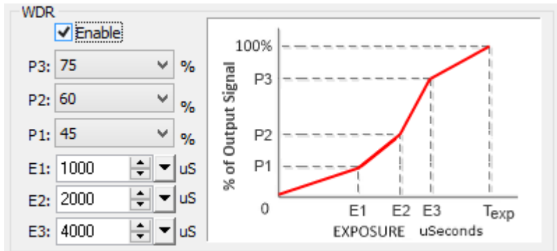
Figure 4.14: Wide Dynamic Range Controls
