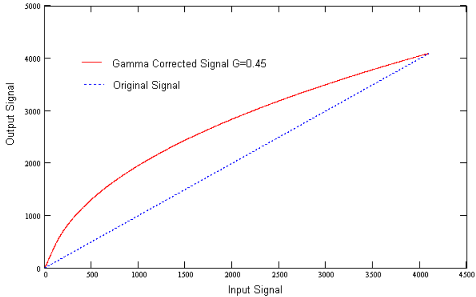
Figure 2.17: Gamma corrected video signal
