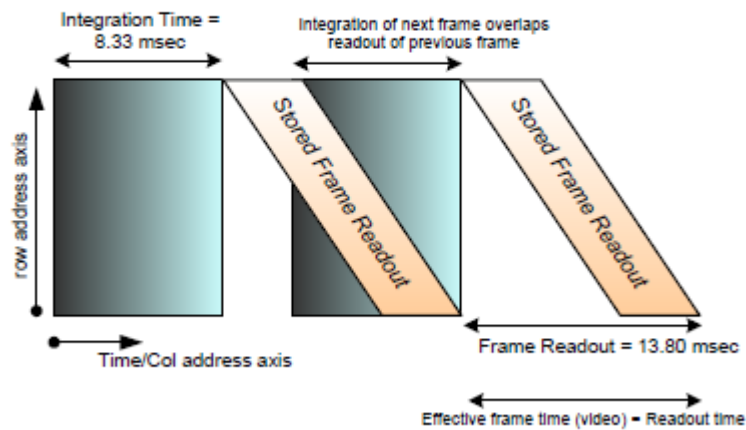
Figure 2.5b: Global Shutter with 8.33mS exposure time
