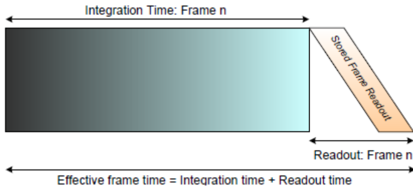
Figure 2.5c: Global Shutter Mode with a long exposure period (integration time)
